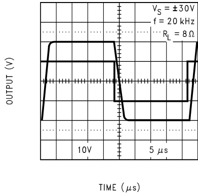
Pulse Response
